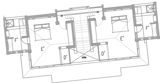
UPPER FLOOR OF VILLA SAYANG
